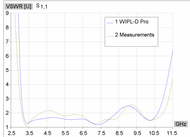
VSWR overlay in range 2.5-11.5 GHz
