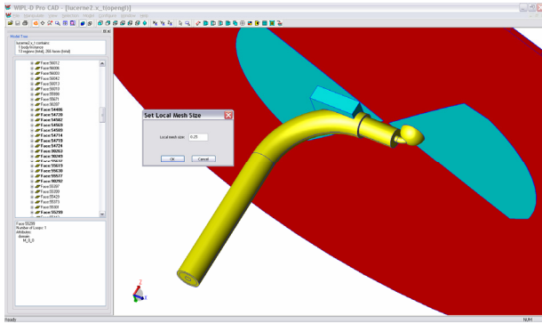
Setting local mesh size
