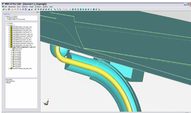
Investigating the inside of the model
