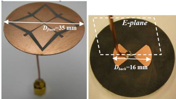
XETS antenna (pictures taken from [1])
