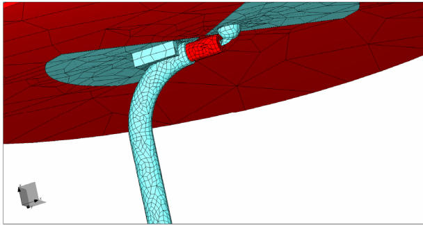
All-quad mesh of XETS model
