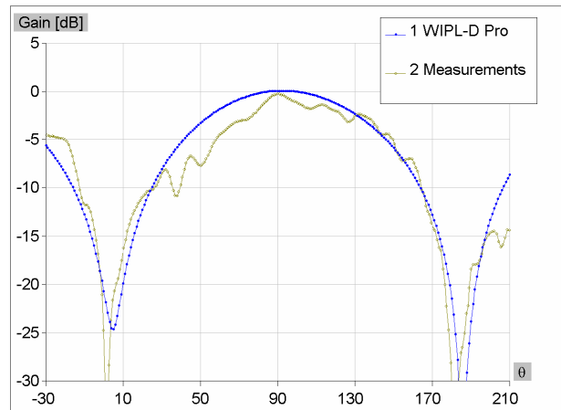
|E| [dB] in E plane 4 GHz
