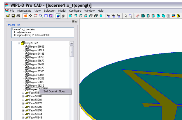
Domain assignment to substrate
