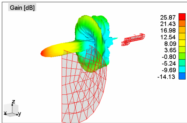
Figure 4. Radiation pattern in 3D
